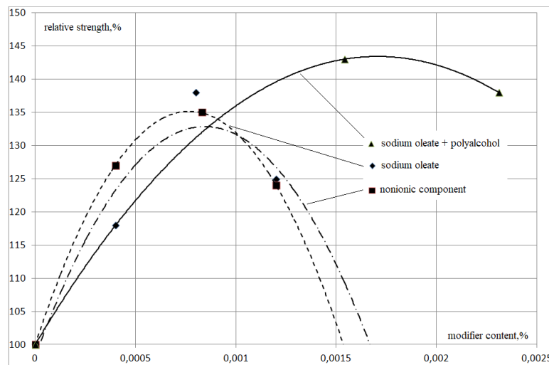
Fig. 3. Relative strength of concrete at the age of 28 days (the strength of concrete without additives is taken as 100%)
