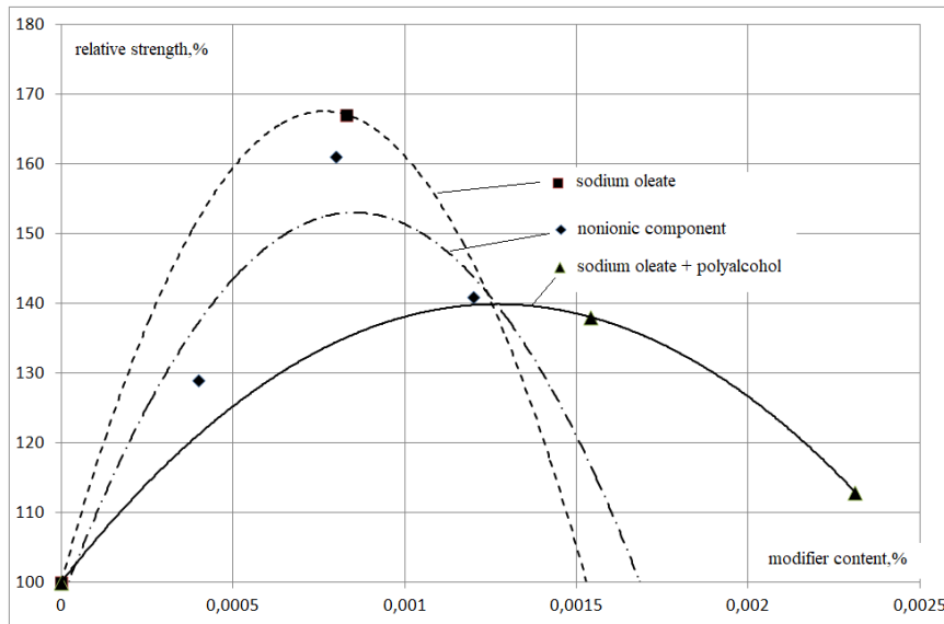
Fig. 2. Relative strength of concrete at the age of 2 days (the strength of concrete without additives is taken as 100%).
